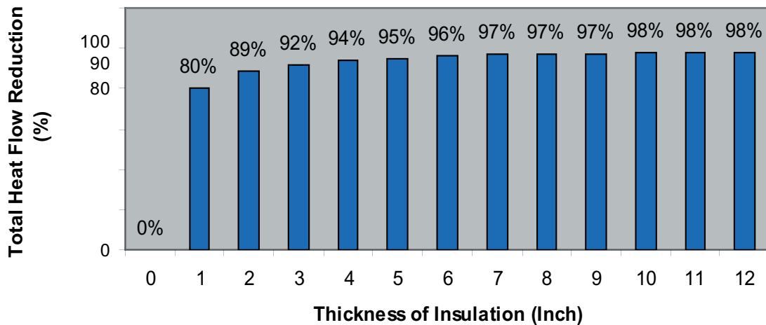
Figure 1.2: Percentage of total heat flow reduction
